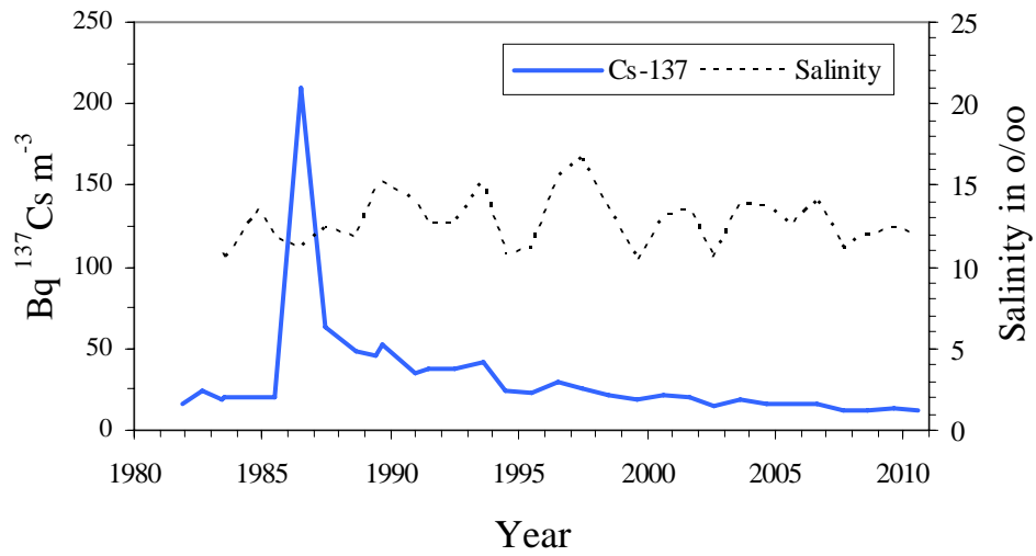
Fig. 4.1. Caesium-137 in seawater collected in Roskilde Fjord 1980 - 2011. (Unit: \text{Bq m}^{-3} )
